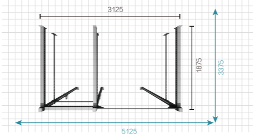
LP6024 DOUBLE WALL MOUNTED RACK
