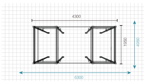
LP6014 THREE-ROWS POWER RACK
